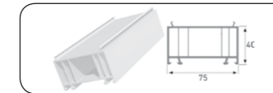
FRAME ELEVATION PROFILE (40 MM)
