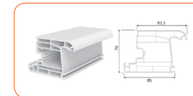
INSIDE OPENING DOOR PROFILE
