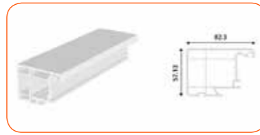
VERTICAL MULLION PROFILE
