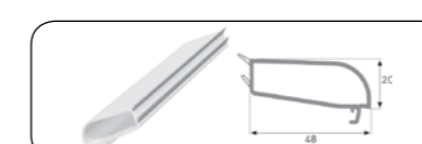
SINGLE GLAZING BEAD PROFILE (5 MM)
