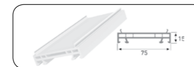
FRAME ELEVATION PROFILE (15 MM)
