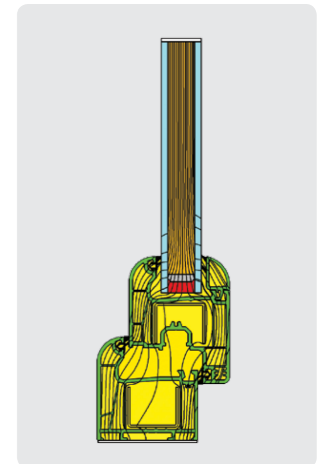
WINDOW HEAT FLOW DIAGRAM UF: 1,46 W/M 2 °K UW: 1,63 W/M 2 °K
