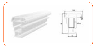
SASH ADAPTING PROFILE
