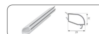
DOUBLE GLAZING BEAD PROFILE (24 MM)
