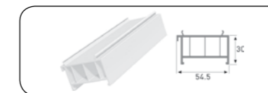
FRAME BASE MONTAGE PROFILE
