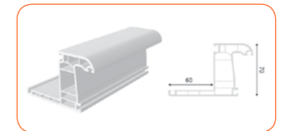
WIDE LINING FRAME PROFILE
