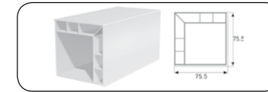
ANGLED POST BOX 90° PROFILE
