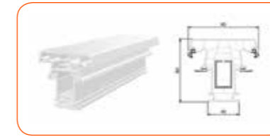
MULLION PROFILE
