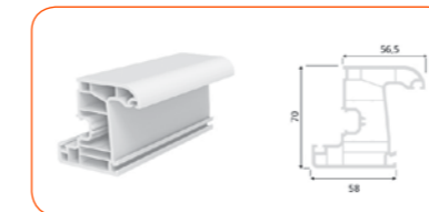
SASH PROFILE
