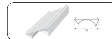
ANGLED POST ADAPTING PROFILE
