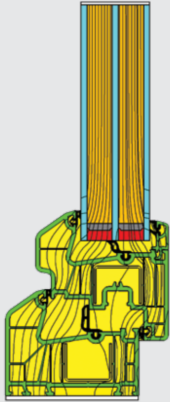
HEAT FLOW DIAGRAM
